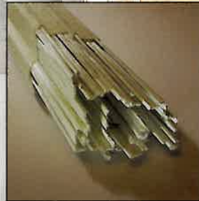
Ultra lineal before it enters the die. Note how the roving and mats work together to add strength in all directions.
